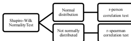
FIGURE 3. Data Analysis Procedure. The data analysis technique uses the Shapiro Wilk test, if the data is normally distributed then it is continued with the r-person test and vice versa.
