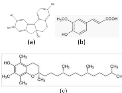
Gambar 1. (a) Brazilein; (b) Phenol; (c) Vitamin E
