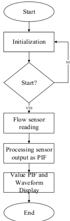
FIGURE 4. The flowcart system in research design of ventilator tester using F1031V sensor
