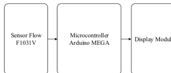
FIGURE 1. The diagram block of the system in research design of ventilator tester using F1031V sensor
