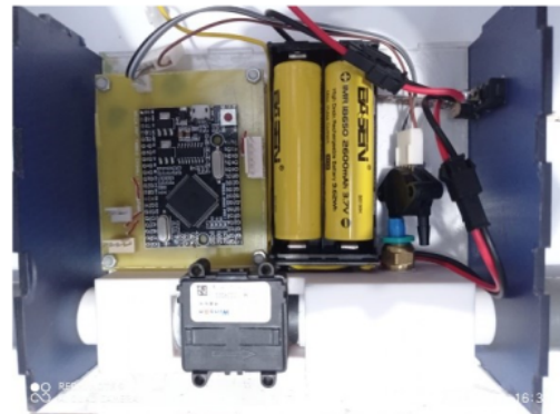
FIGURE 3. overall circuit ventilator tester using sensor F1031V
