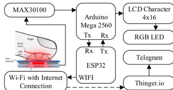
FIGURE 1 Diagram Block
