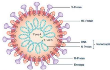
Fig. 1 Coronavirus.
