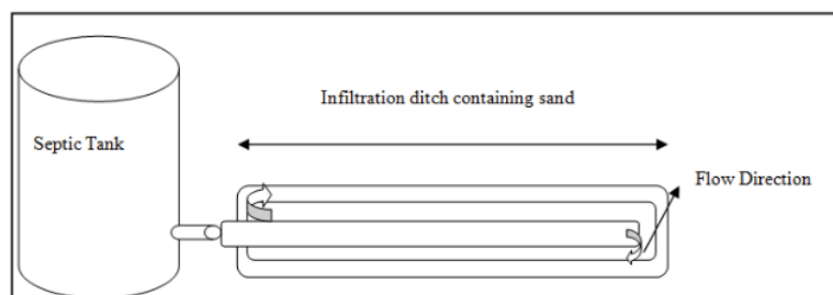
Fig. 1. Tripikon Infiltration Design
