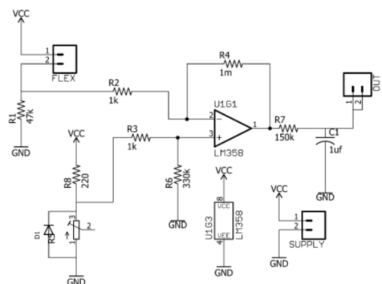
Fig. 4. Differential Amplifier
