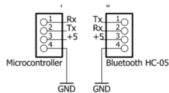
Fig. 5. Bluetooth Connection
