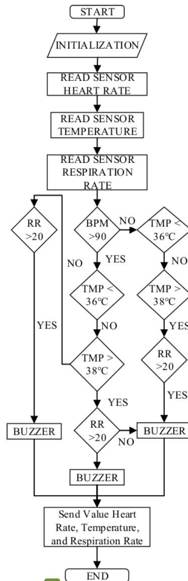
Fig. 2. The flowchart of the Arduino Program
