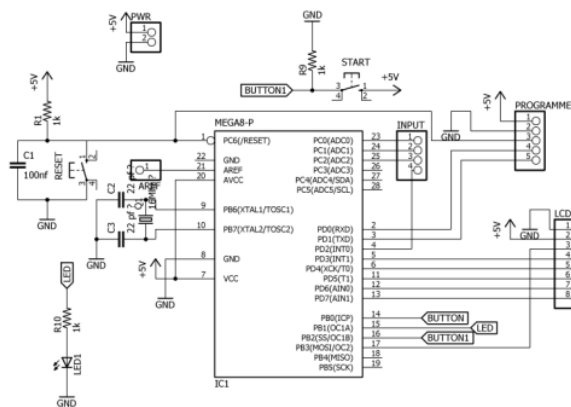
Fig. 6. Minimum System Circuit
