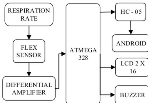
Fig. 1. Block Diagram Parameters Respiration Rate
