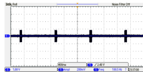
Fig. 15. Output From circuit Differential Amplifier Input Current
